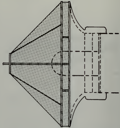
FIGURE 2-23. Bellmouth compressor inlet.
